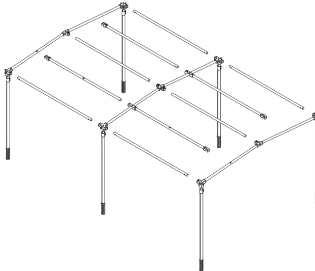
Figure 2 - Assembly diagram
