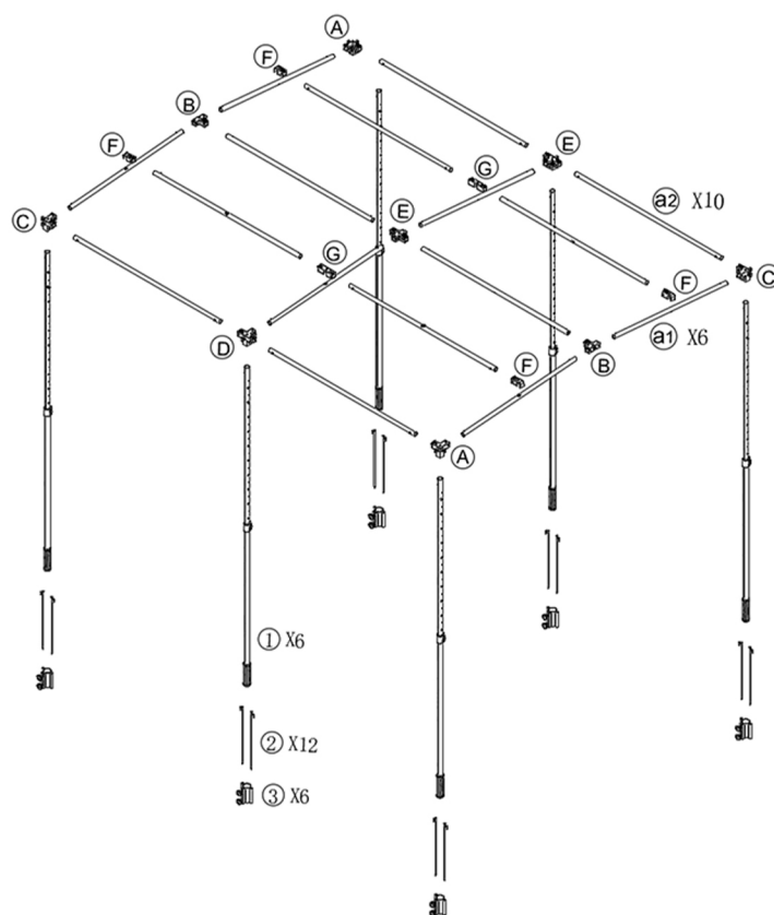
SC24 Exploded View-1
