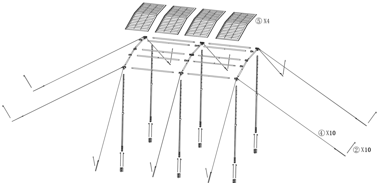
SC24 Exploded View-3
